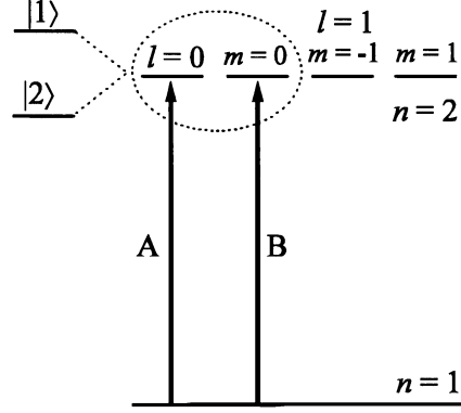
Figure 3. A spinless model of the hydrogen atom. The information channel is made of the input forbidden nlm \rightarrow n'l'm' transition 100–200 and the output dipole active 100–210 transition.
