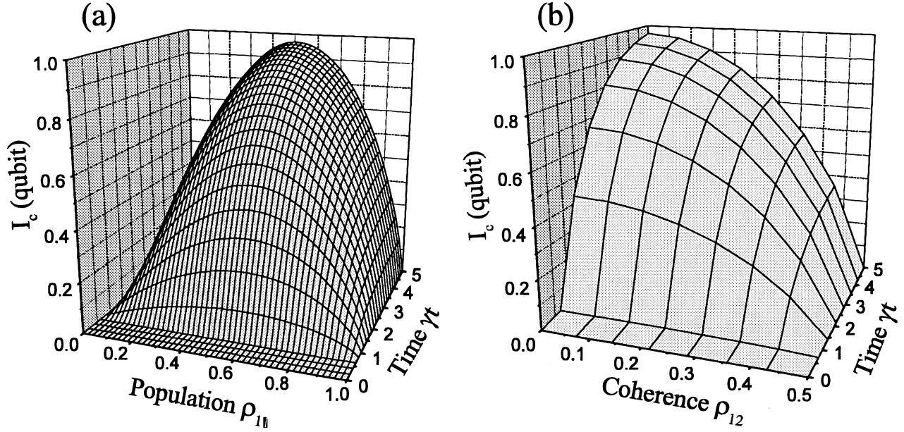
Figure 6. The coherent information transmitted in the atom-to-field quantum channel versus the dimensionless time \gamma t and input atomic density matrix, which is taken either diagonal with the ground state matrix element \rho_{11} (a) or as the sum of \hat{I}/2 and the real (“cosine-type”) coherent contribution of the off-diagonal elements \rho_{12}\hat{\sigma}_1 (b).
