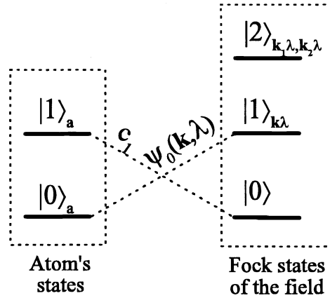
Figure 5. Structure of the joint Hilbert space of the (atom+field) system. For the vacuum initial field state, both atomic states and only two Fock states of the field ( |0\rangle and |1\rangle ) are involved in the dynamics of the joint system (atom+field). The dynamics is entirely defined by just two states, |0\rangle_a |1\rangle_{k\lambda} and |1\rangle_a |0\rangle , which are described by \psi_0(\mathbf{k}, \lambda) and c_1 , respectively.
