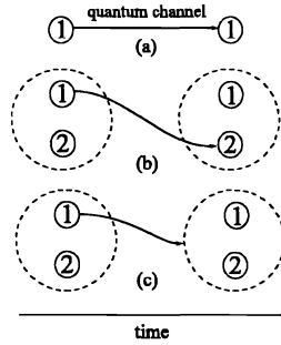
Figure 1. Classification of possible quantum channels connecting two quantum systems. 1 \rightarrow 1 , information is transmitted from the initial state of the system to its final state (a); 1 \rightarrow 2 , information is transmitted from subsystem 1 of the system (1+2) to subsystem 2 of the system (b); 1 \rightarrow (1 + 2) , information is transmitted from subsystem 1 of the system (1+2) to the whole system (1+2) (c).
