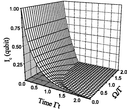
Figure 2. The coherent information transmitted between the states of the TLA at two time instants, t = 0 and t > 0 , versus time \Gamma t and the Rabi frequency \Omega/\Gamma (both are dimensionless).
