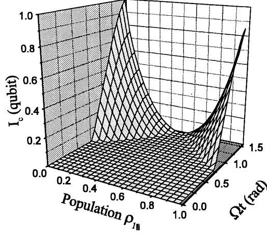
Figure 4. The coherent information transmitted between two unitary coupled TLAs versus population \rho_{11} of the diagonal initial density matrix of the second TLA and the coupling precession angle \Omega t .
