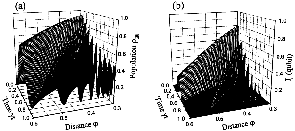
Figure 7. Excited state population of the second atom (a) and the coherent information (b) in a system of two atoms interacting via the free space field versus time \gamma t and the interatomic distance \varphi = \omega_0 R/c (both are dimensionless). The input density matrix is diagonal with the ground state matrix element \rho_{22} = 1/2 .
