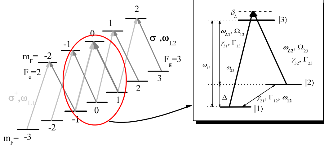
Figure 1. \Lambda systems formed of the Zeeman sublevels in the F_g = 3 \rightarrow F_e = 2 transitions excited by the \sigma^+ and \sigma^- components of the respective frequencies \omega_1 and \omega_2 , whose difference is equal to the splitting of the Zeeman sublevels with \Delta m_F = 2 . Three-level system in \Lambda -configuration has the following parameters: \omega_{L1}, \omega_{L2} are the frequencies of the laser fields driving transitions of the system; \Omega_{13}, \Omega_{23} are the respective Rabi frequencies; \delta_L is the frequency detuning from the |1\rangle \leftrightarrow |3\rangle transition; \gamma_{31}, \gamma_{32} are the decay rates from excited state |3\rangle onto the low-lying levels |1\rangle and |2\rangle ; \gamma_{12} and w are the decay and pumping rates of the level |1\rangle via the level |2\rangle , correspondingly; \Gamma_{31}, \Gamma_{32} , and \Gamma_{12} are the dephasing rates for the transitions |1\rangle \leftrightarrow |3\rangle and |2\rangle \leftrightarrow |3\rangle , and |1\rangle \leftrightarrow |2\rangle , respectively.
